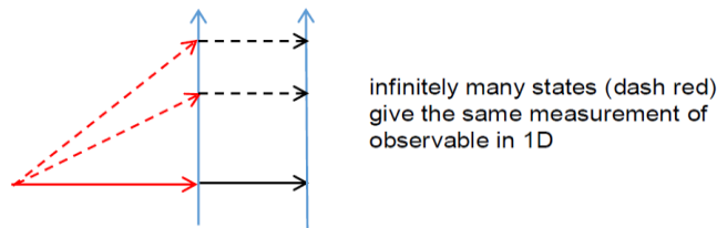
Fig.2.2. State acts in two dimensions though the result is available just as projection
