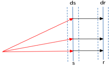
Fig.2.3. Probabilistic distribution of states results in probabilistic measurements
