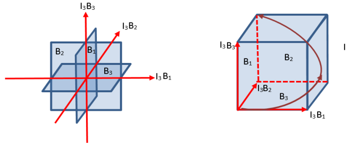
Fig.3.2. Basis of bivectors and unit value pseudoscalar
