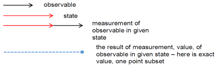
Fig.2.1. A state acts on observable in one-dimensional movement
